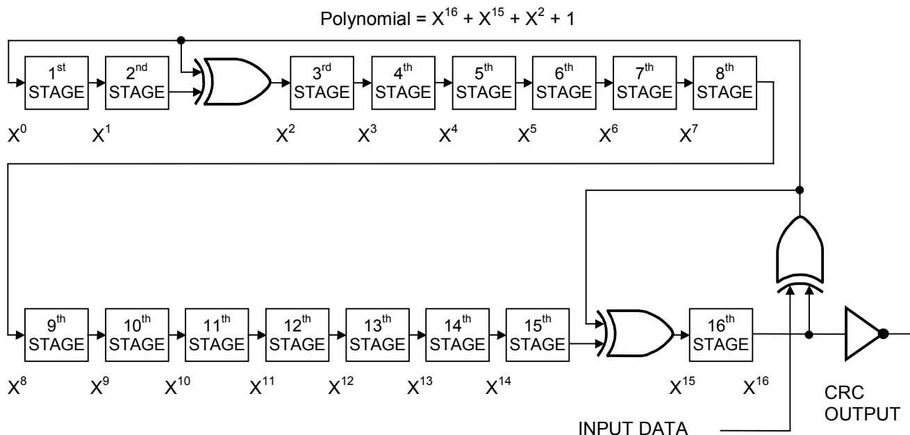
Figure 12. CRC-16 HARDWARE DESCRIPTION AND POLYNOMIAL
